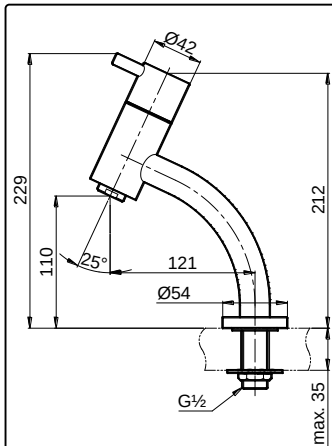
TX 125 LES "EGO II" Lavatory Faucet (Height= 110 mm)
