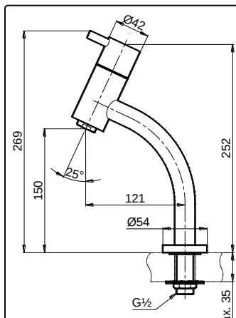
TX 125 LESV1 "EGO II" Extended Lavatory Faucet (Height= 150 mm)
