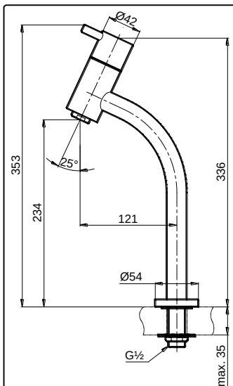
TX 125 LESV2 "EGO II" Extended Lavatory Faucet (Height= 234 mm)
