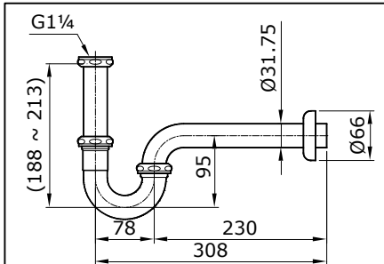
THX1A-5N P-Trap for Lavatory (L=308 mm) For 1 1/4" Pop Up Waste Lavatory Faucet
