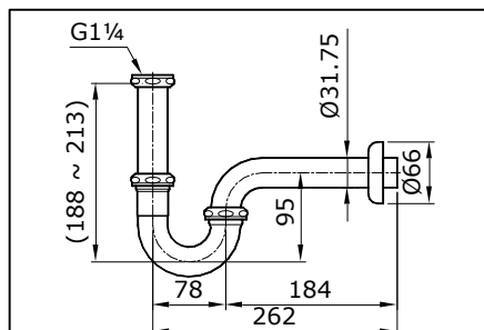
THX1A-3N P-Trap for Lavatory (L=262 mm) For 1 1/4" Pop Up Waste Lavatory Faucet
