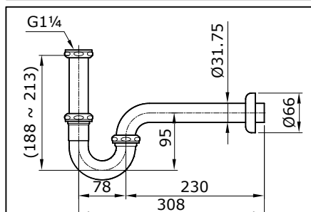
THX1A-5N P-Trap for Lavatory (L=308 mm) For 1 1/4" Pop Up Waste Lavatory Faucet
