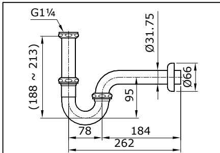
THX1A-3N P-Trap for Lavatory (L=262 mm) For 1 1/4" Pop Up Waste Lavatory Faucet
