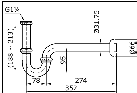
THX1A-6N P-Trap for Lavatory (L=352 mm) For 1 1/4" Pop Up Waste Lavatory Faucet
