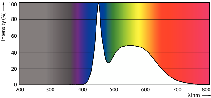
Spectral Power Distribution Colour - TForce Core HB 50W E40 865 GN3
