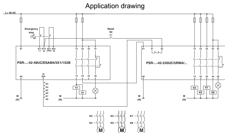
Two-channel emergency stop monitoring with contact extension
